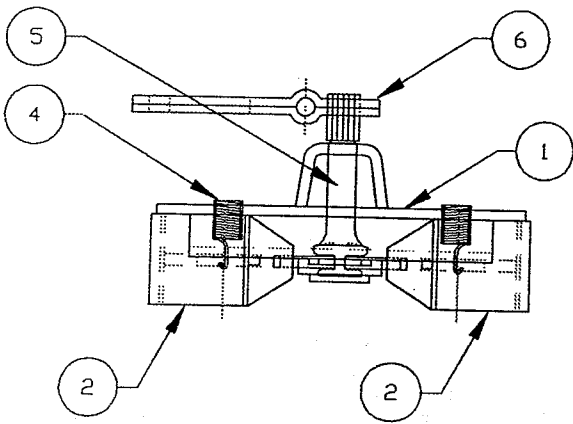
BRAKE/CAM/LEVER/BACKING PLATE ASSY.
