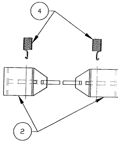
BRAKE SHOE / HOLD DOWN SPRING DETAIL
