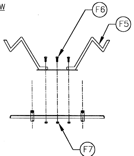
HOSE HANGER SUPPORT BRACKET
