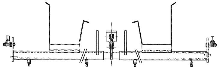
C BRAKE SLEEVE ASSEMBLY SECTION 5.2.3-C
