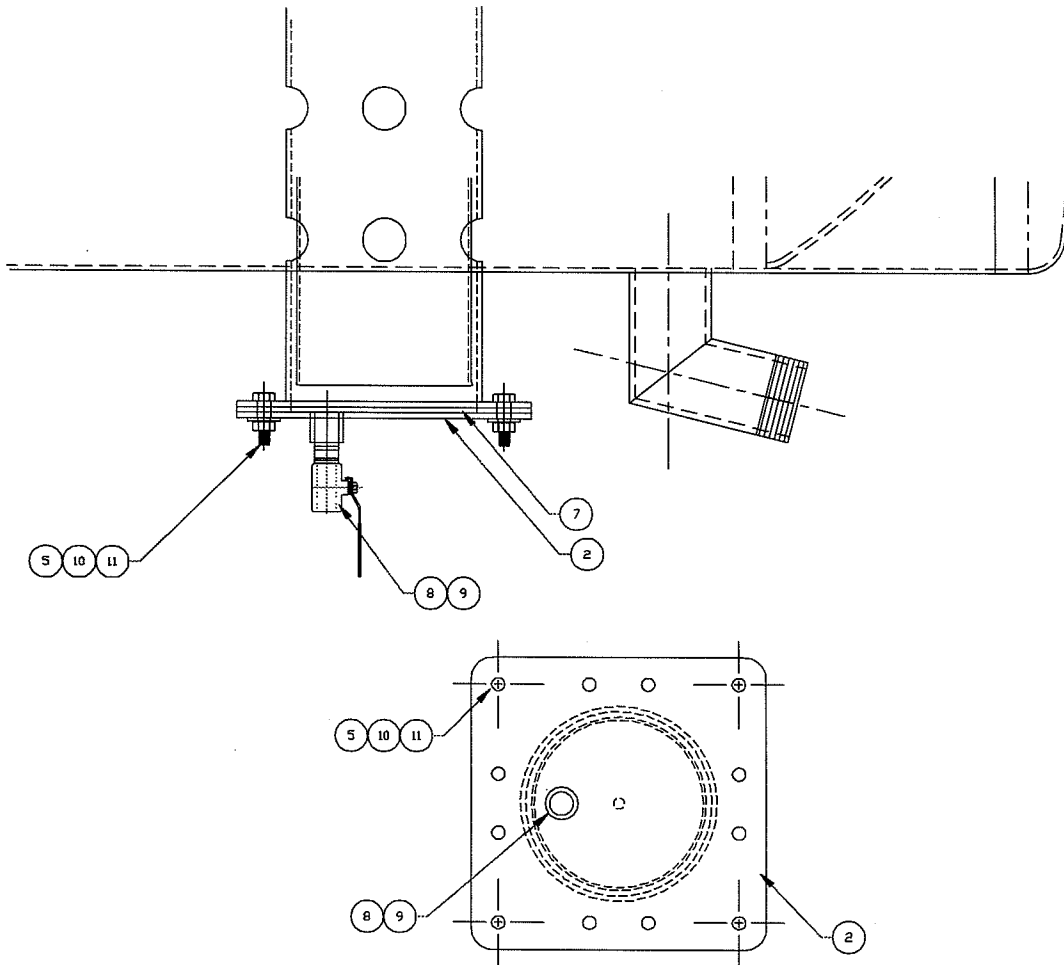
MATING FLANGE AND ASSEMBLY DETAILS
