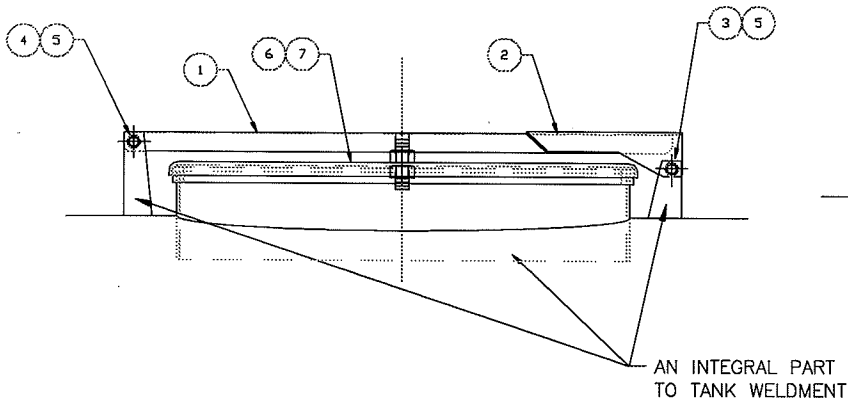
ASSEMBLED DETAIL
