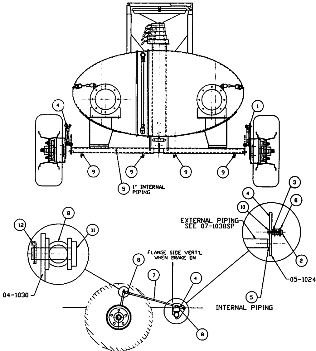
ASSEMBLY No. 08-1008SP MAJOR ASSEMBLY- BRAKE ASSEMBLY
