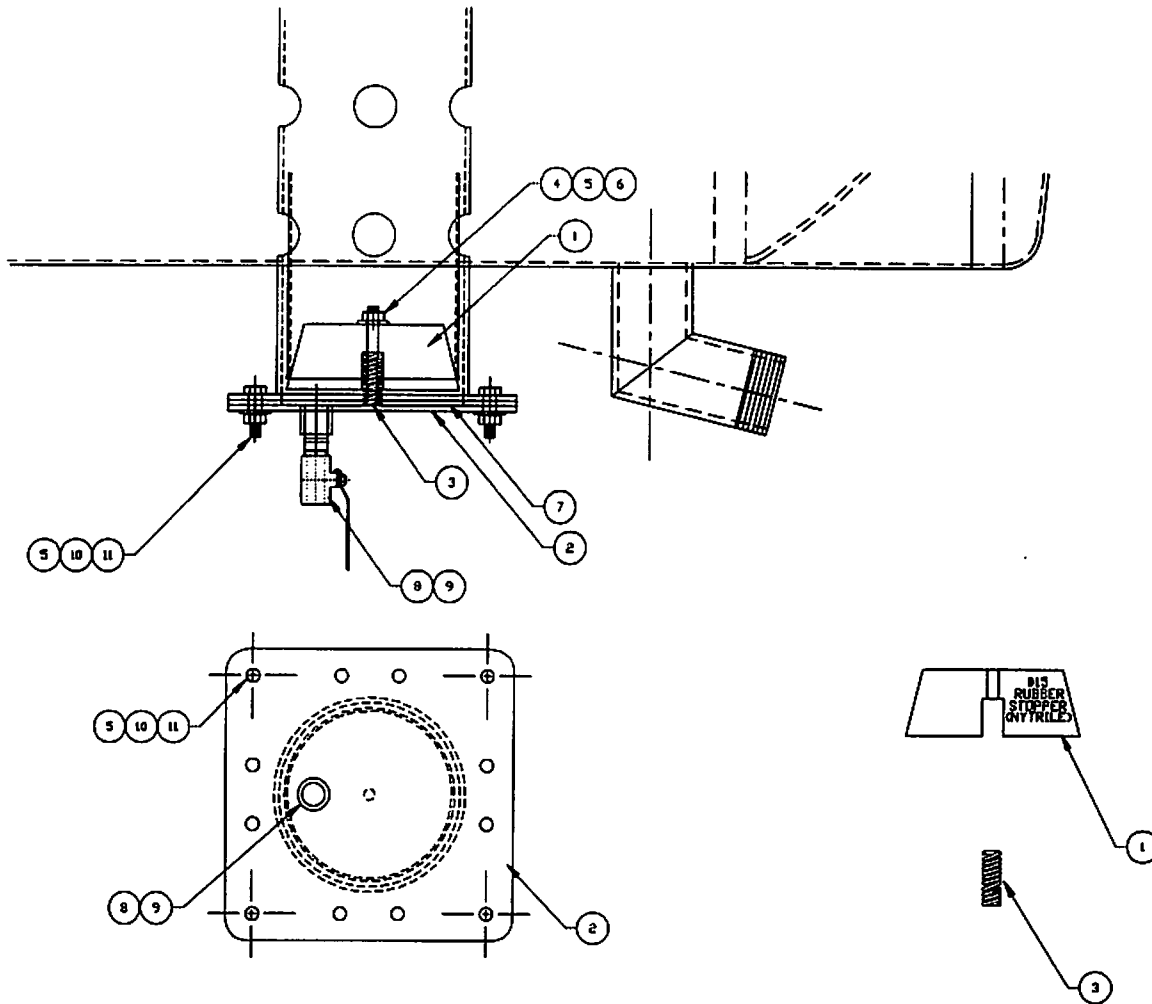
MATING FLANGE AND ASSEMBLY DETAILS
