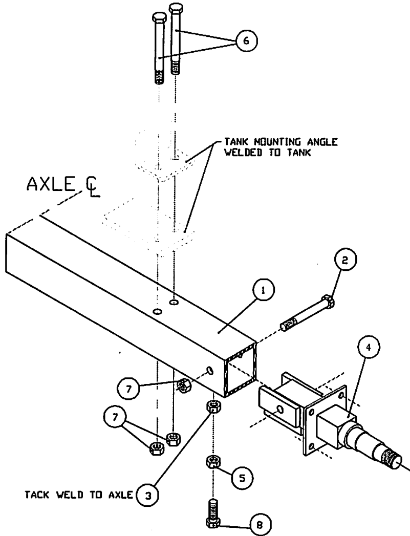
ASSEMBLY No. 08-10102 MAJOR ASSEMBLY- AXLE ASSEMBLY
