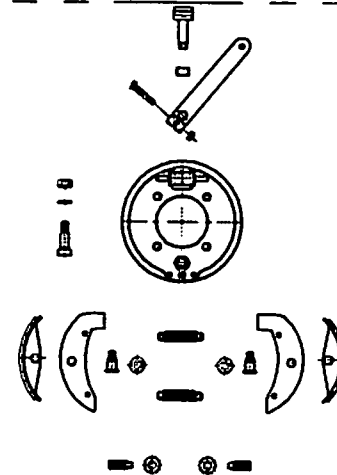
(B) BRAKE ASSEMBLY SECTION 5.2.3-B
