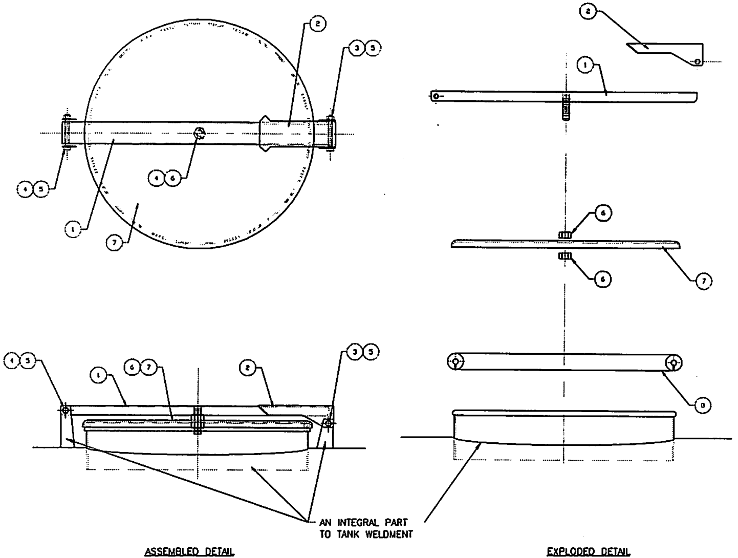
ASSEMBLED DETAIL
