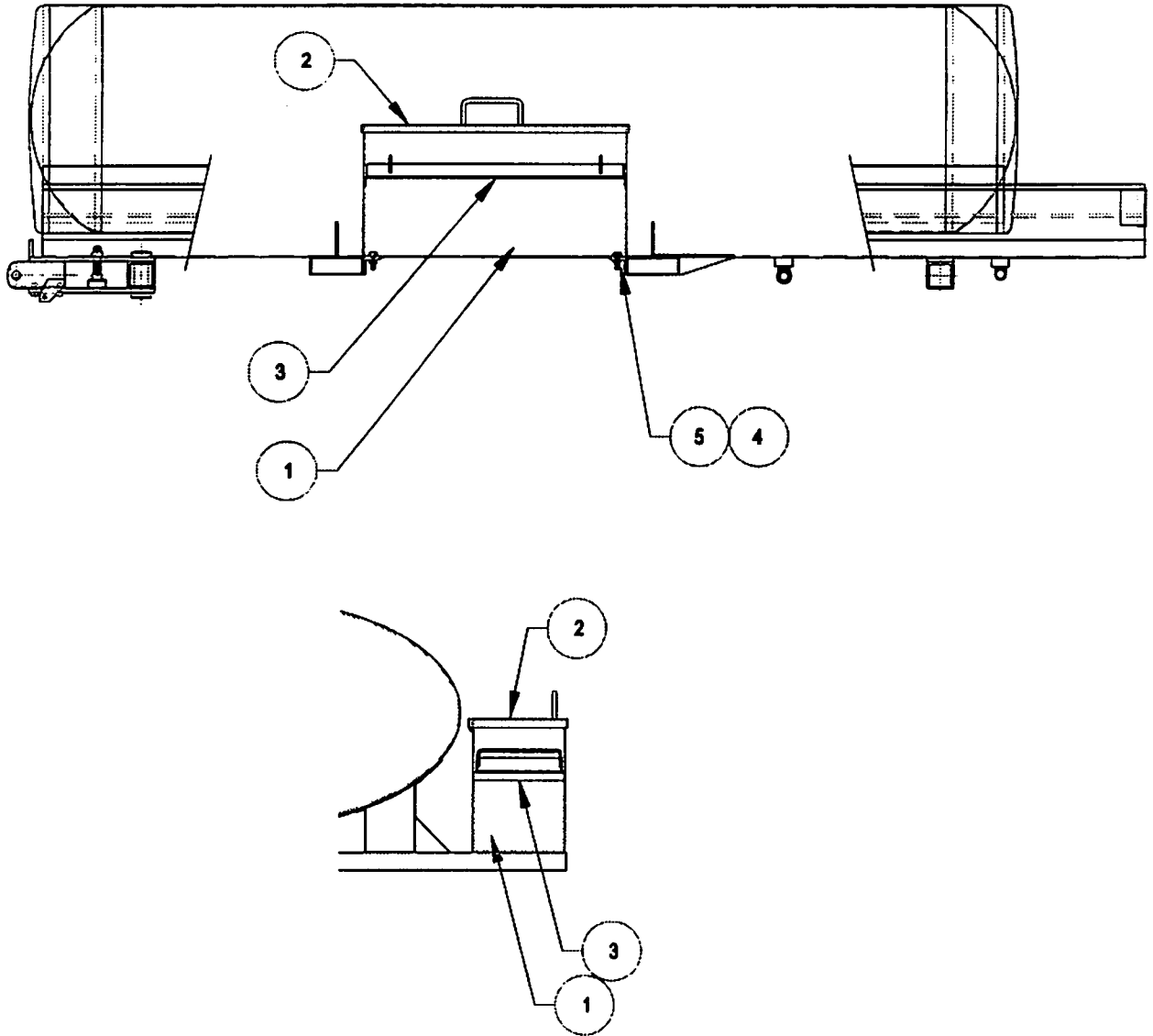
ASSEMBLY No. SMP15575TB MAJOR ASSEMBLY- TOOL BOX
